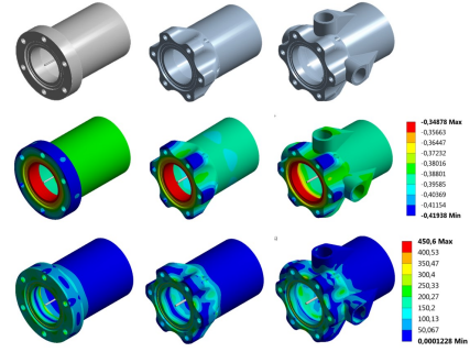
Figure 1: Topological optimisation of the BPM. The left column correspond to the original BPM, the center column to the end of the i3D BPM not on the feedthrough side and the right column the i3D BPM on the feedthrough side. The top line shows a view of the CAD model, the middle line show the stress induced displacement in millimeters when the BPM is bolted and the bottom line the Von Mises strains in MPa.
